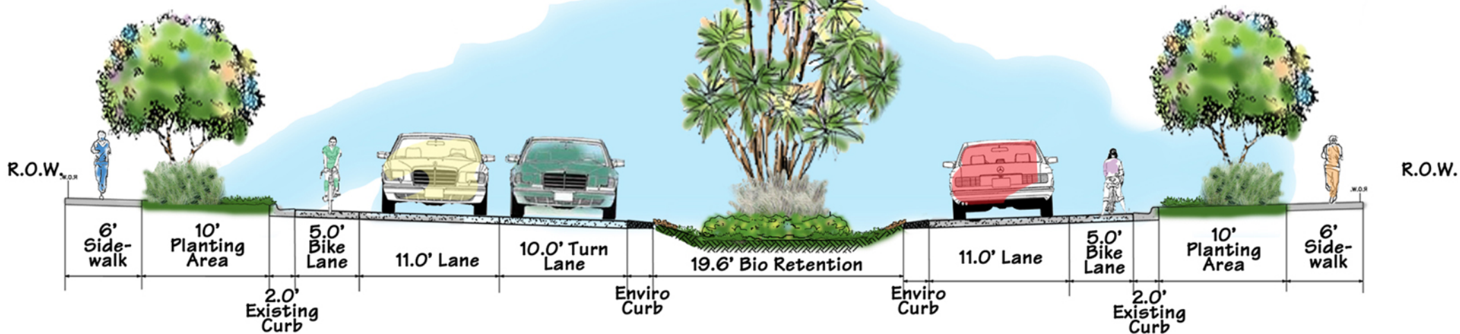
Concept #2- Proposed Roadway Section widen medians-add turn lanes
